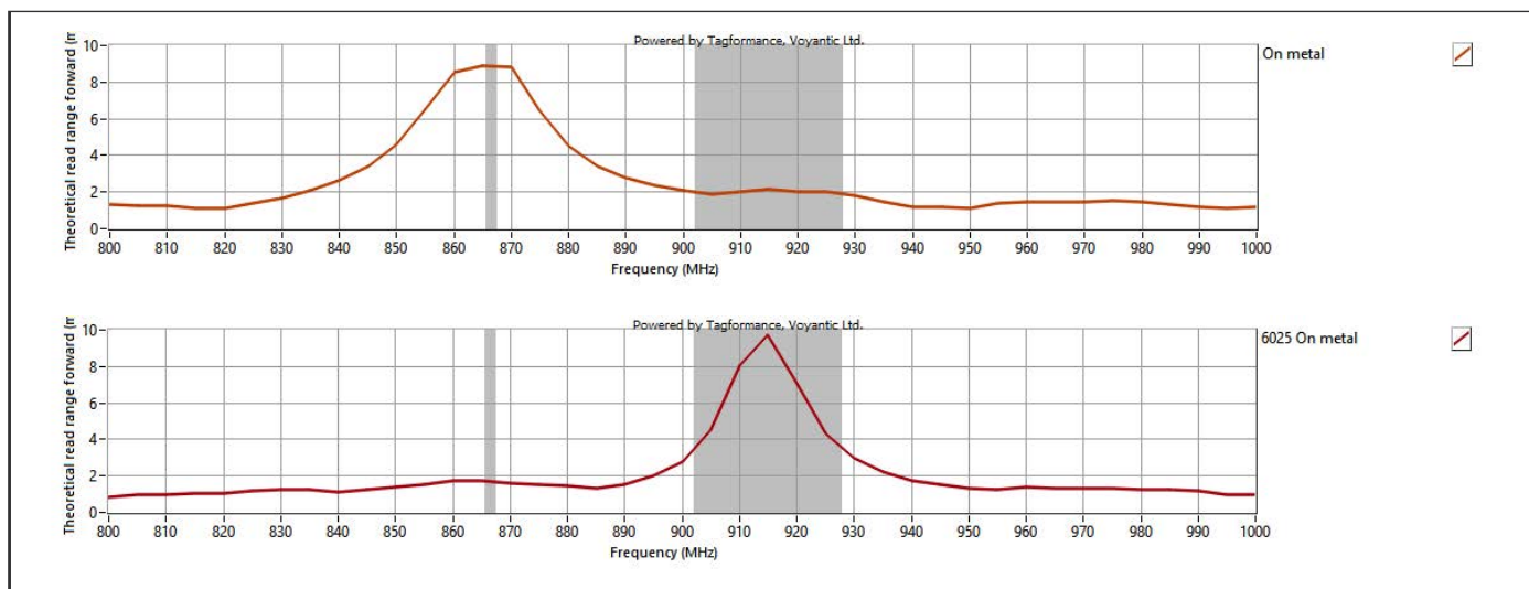
UNI 6025 - RF performance
